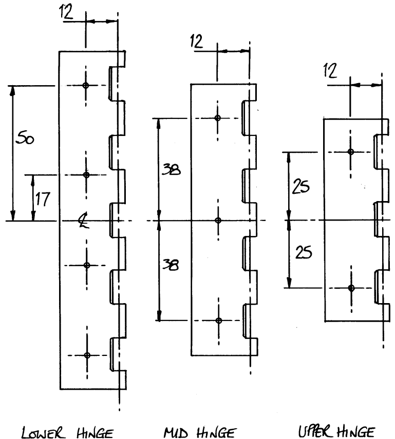
Fig 3. Rudder hinge bolt attachment hole locations.
