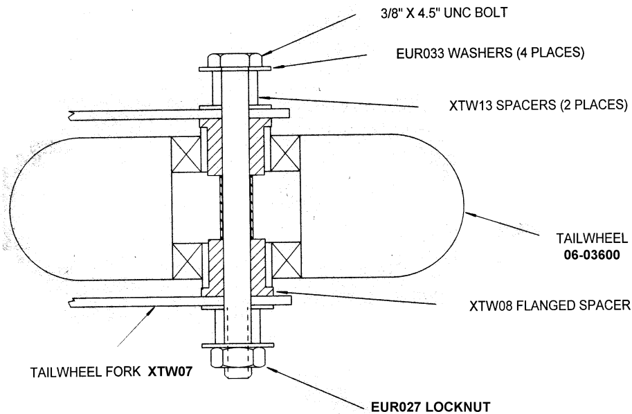
Fig 6. Section through tailwheel axle.
