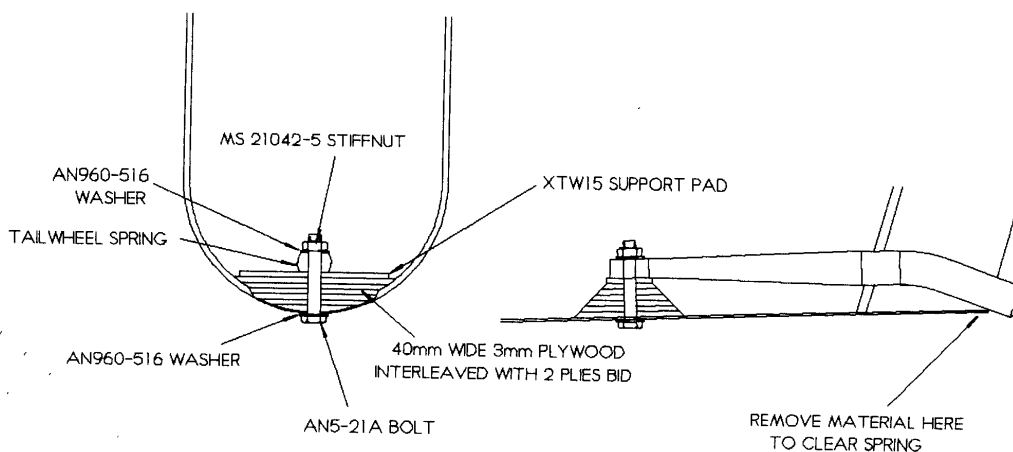
Fig 4. Forward mounting of tailwheel spring.
