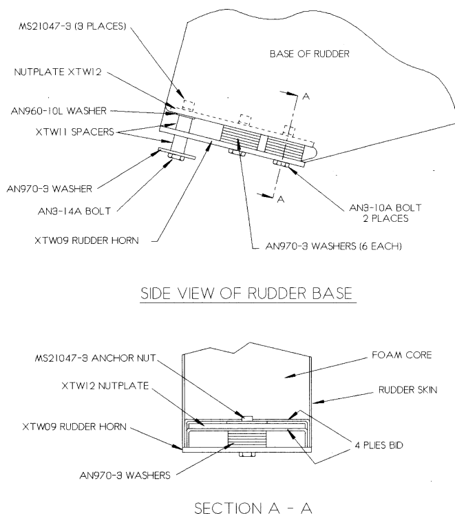
Fig 7. Cable mountings.
