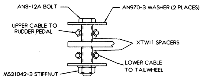
Fig 9. Detail of starboard cable fixing.
