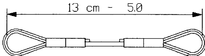
Fig 8. Tailwheel drive cable.
