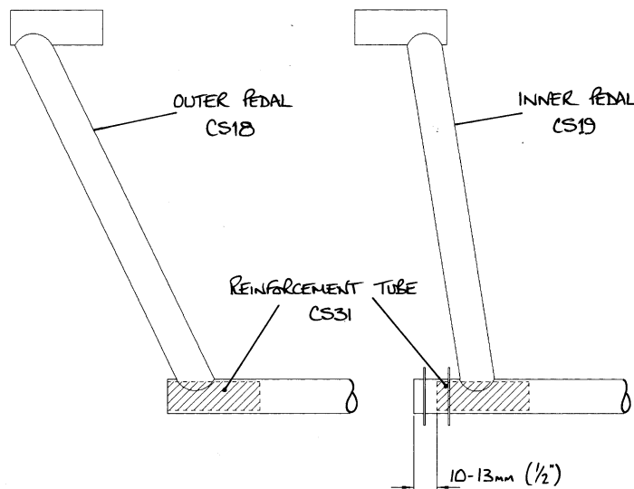
Fig 3. Rudder pedal tube reinforcement.
