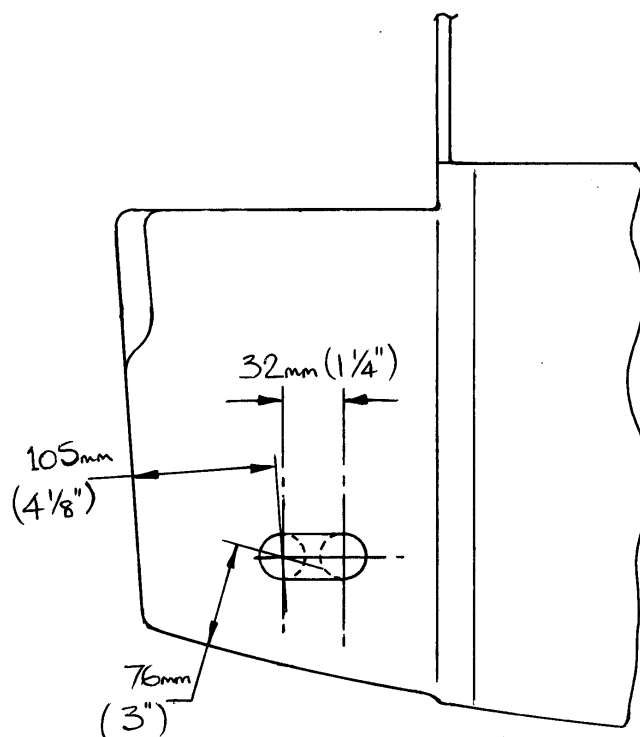
Fig 2. Slot for rudder pedals. Inboard face stbd footwell shown
