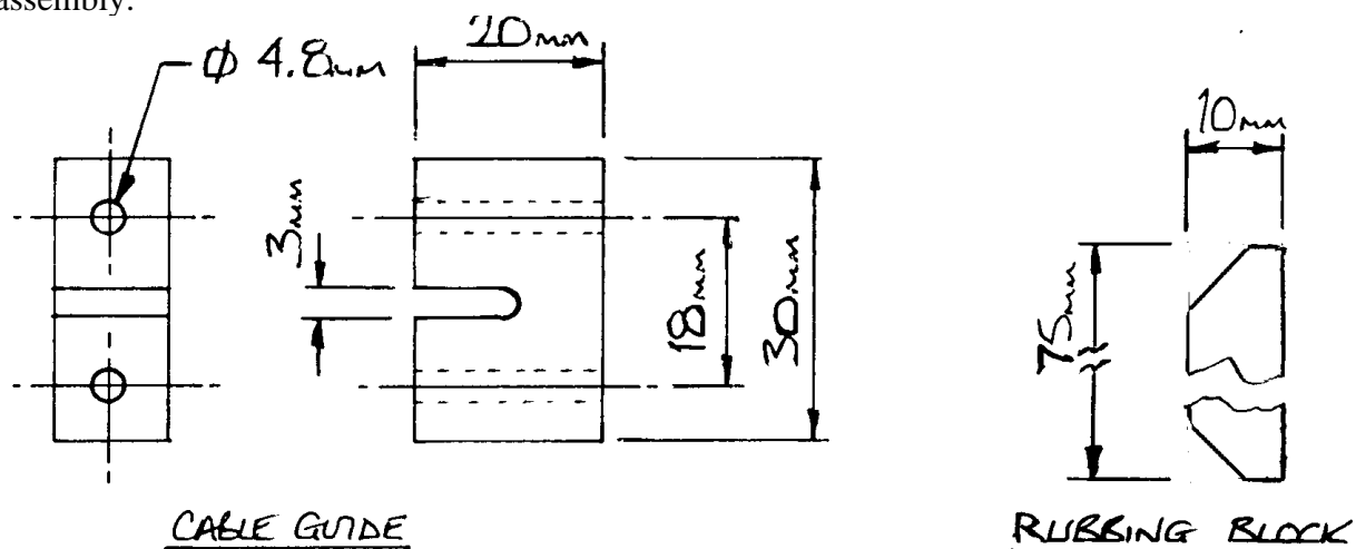
Fig 6. Cable guide and rubbing block.
