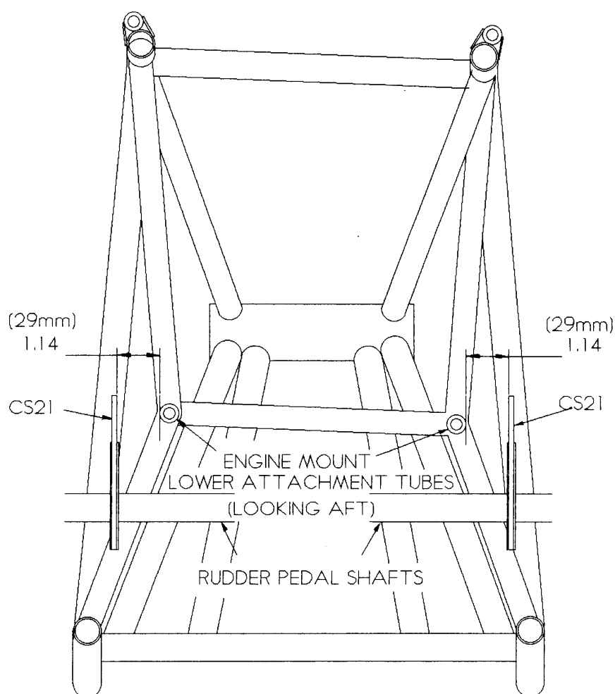
Fig. 4. Pedal lateral alignment (monowheel frame shown).
